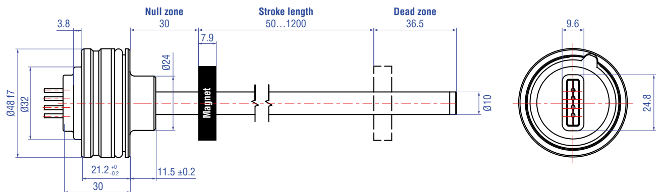
Fig. 4: Tempsonics® MH-Series MH sensor, part 1
