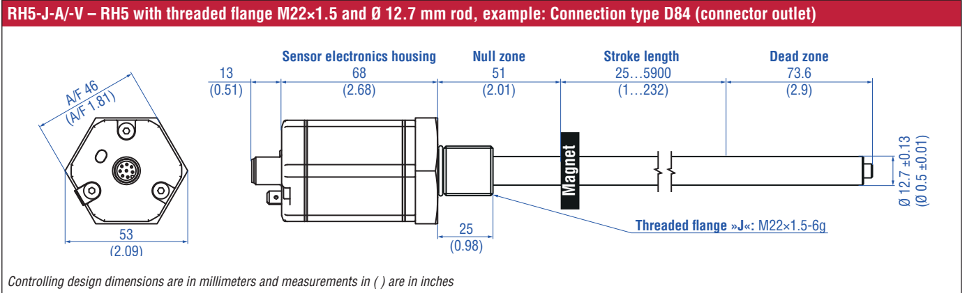
Fig. 3: Temposonics® RH5 with ring magnet, part 2
