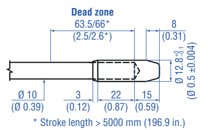
Fig. 2: Temposonics® RH5 with ring magnet, part 1
