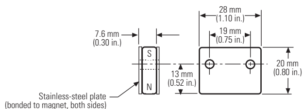
Floating magnet, style M part no. 251298-2
