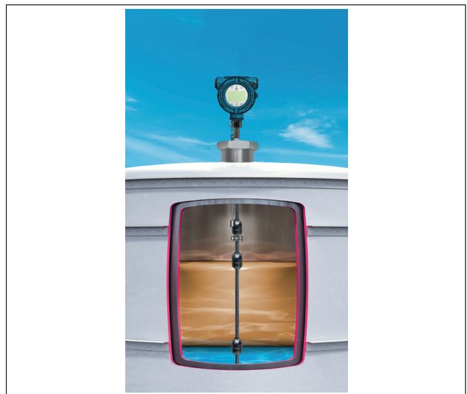
Fig. 3: Example of product and interface level measurement
