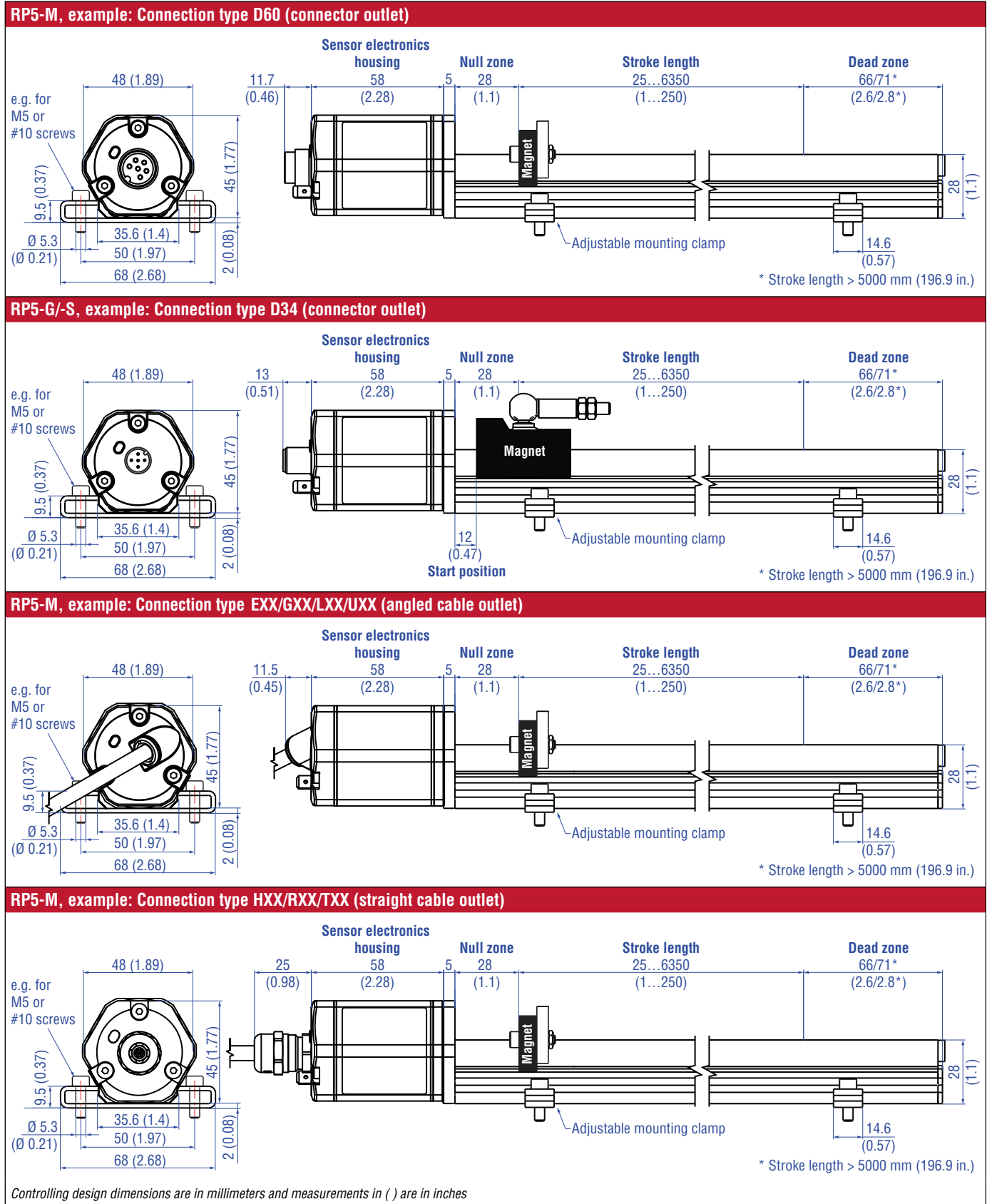
Fig. 2: Temposonics® RP5 with U-magnet/magnet slider
