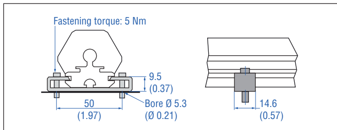
Fig. 10: Mounting clamps (part no. 400 802) with cylinder screw M5x20
