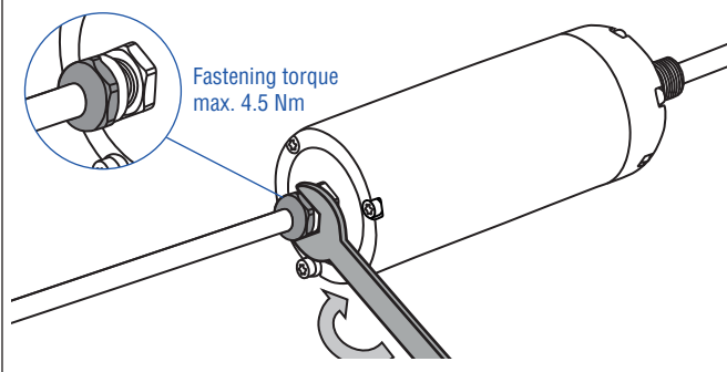
Fig. 56: Replacement of the base unit on model RM5, part 4
