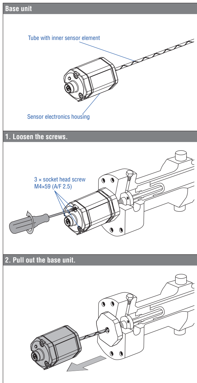
Fig. 50: Replacement of the base unit (e.g. RH5 sensor), part 1
