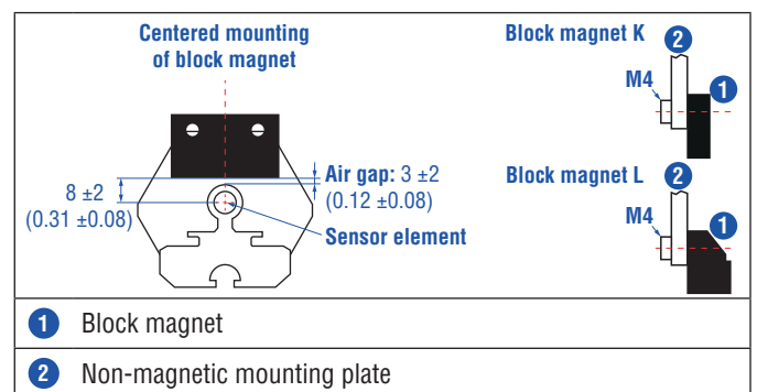
Fig. 38: Mounting of block magnet K (part no. 251 298-2) and block magnet L (part no. 403 448)
