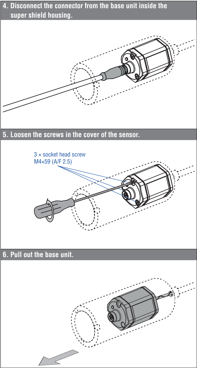
Fig. 54: Replacement of the base unit on model RM5, part 2
