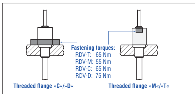
Fig. 28: Mounting example of threaded flange »C«/»D«, »M«/»T«
