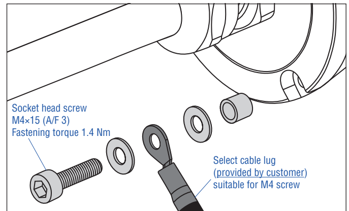
Fig. 58: Installation example for grounding of RM5 sensor
