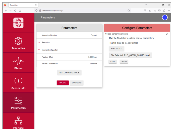
Fig. 83: Uploading a cek file to an R-Series V Analog sensor with the same stroke length
