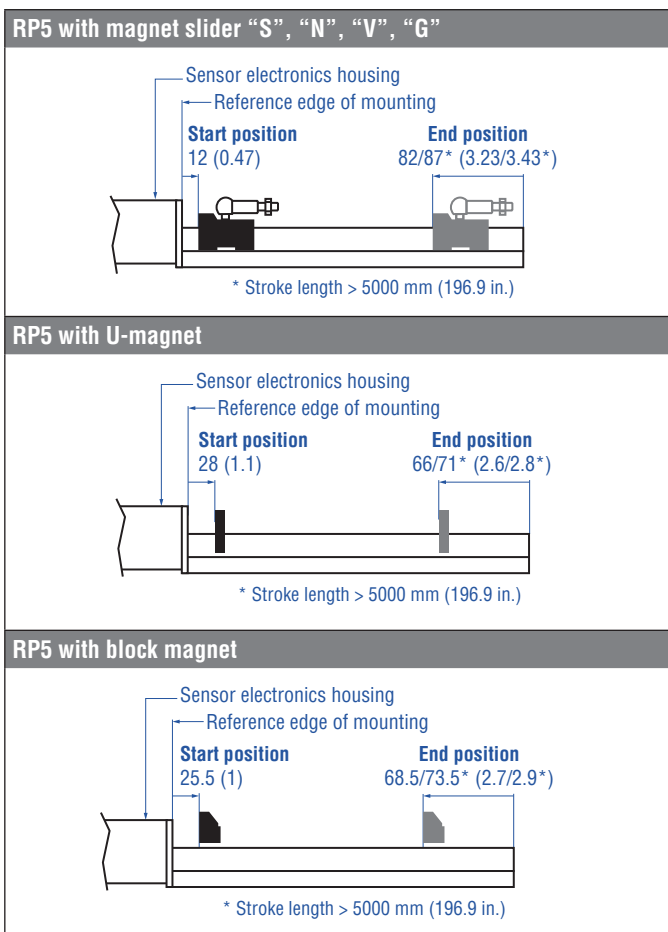
Fig. 41: Start- and end positions of magnets for RP5
