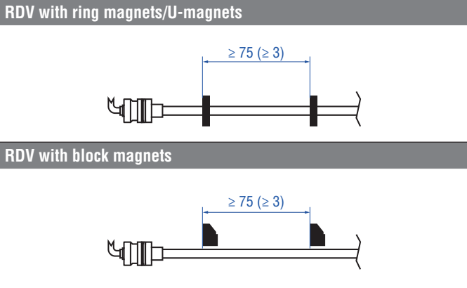
Fig. 49: Minimum distance between magnets for differential/multi-position measurement (RDV)
