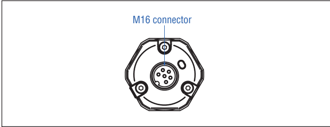
Fig. 59: Location of connection (example M16 connector outlet)
