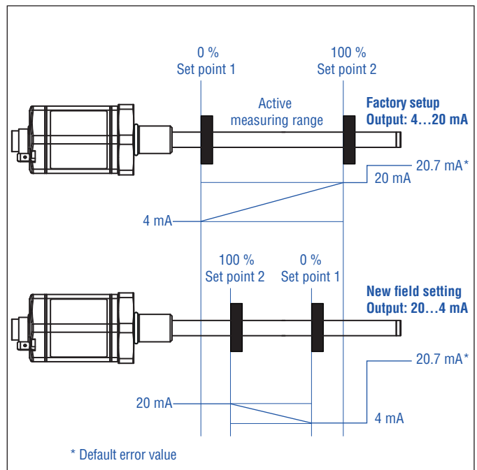
Fig. 68: Reversal of the measuring direction by adjusting the start value (set point 1) and the end value (set point 2)
