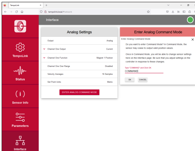
Fig. 85: Start Command Mode
