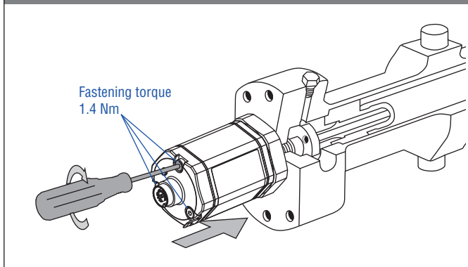
Fig. 51: Replacement of the base unit (e.g. RH5 sensor), part 2
