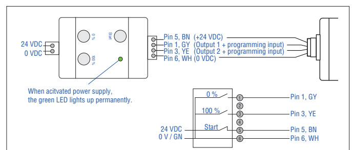
Fig. 88: Connect hand programmer
