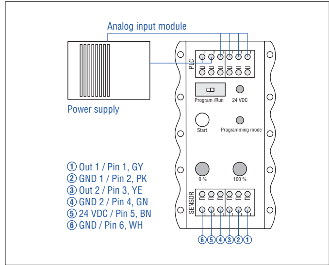
Fig. 90: Connect cabinet programmer
