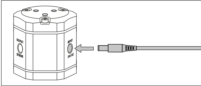
Fig. 73: Connection of power supply to the TempoLink® smart assistant
