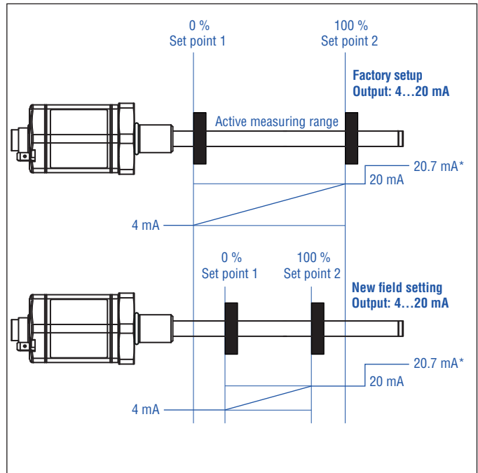
Fig. 67: Shifting the start position (set point 1) and end position (set point 2)
