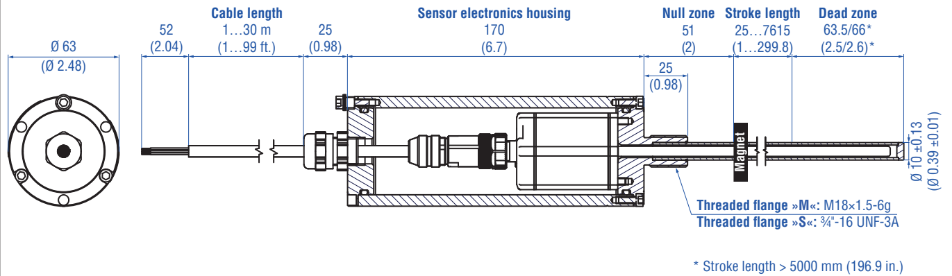
Fig. 12: Temposonics® RM5 with ring magnet
