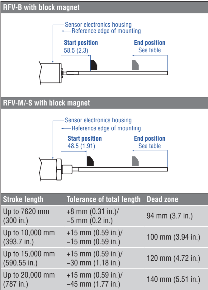
Fig. 45: Start- and end positions of magnets for RFV with block magnet
