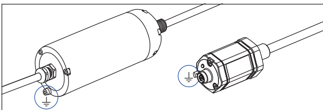
Fig. 57: Grounding via ground lug on the example of an RM5 sensor (left) / RH5 sensor (right)
