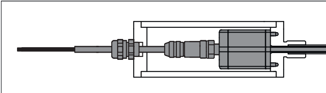
Fig. 52: Base unit in the super shield housing of the RM5
