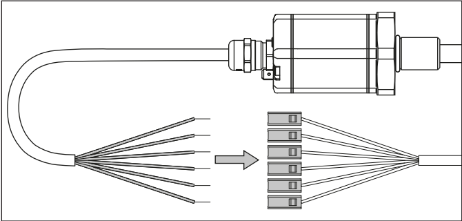
Fig. 72: Connection of adapter cable to R-Series V sensor with cable outlet
