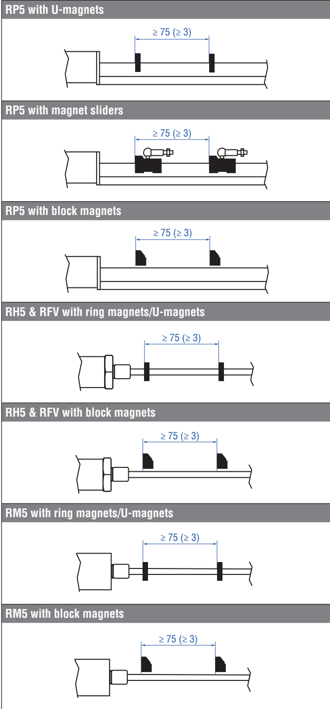
Fig. 48: Minimum distance between magnets for differential/multi-position measurement (RP5, RH5, RFV, RM5)
