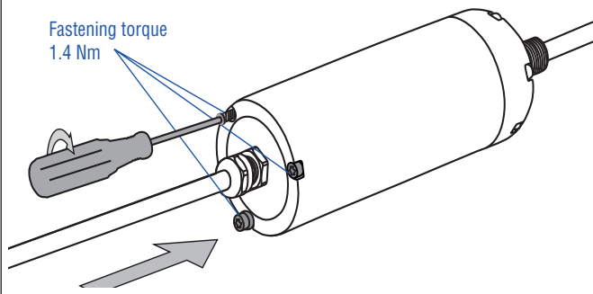
Fig. 55: Replacement of the base unit on model RM5, part 3
