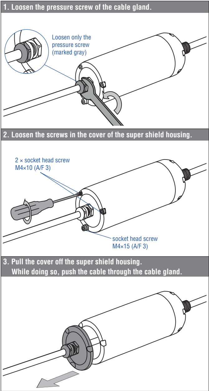
Fig. 53: Replacement of the base unit on model RM5, part 1
