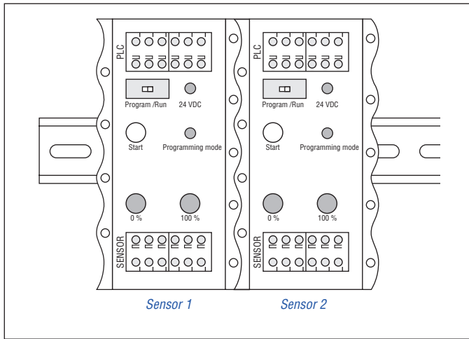
Fig. 89: Installation of cabinet programmer on a 35 mm standard rail
