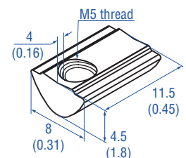
T-nut Part no. 401 602
