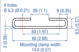
Mounting clamp Part no. 400 802
