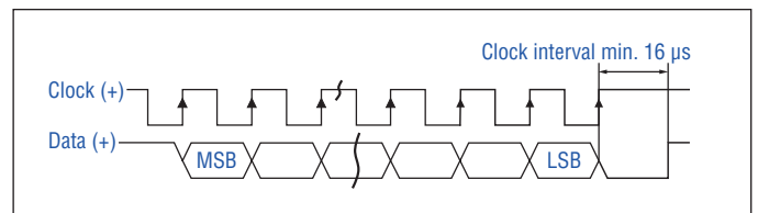
Fig. 24: Timing diagram
