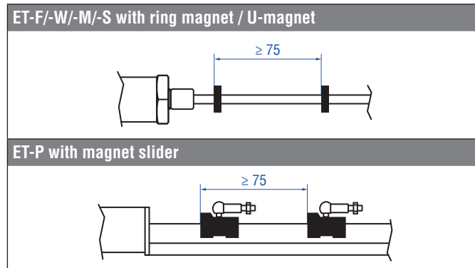
Fig. 18: Examples: Minimum distance for multi-position measurement
