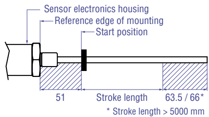
G-Series GT2 / GT3 with U- / ring-magnet
