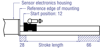
G-Series GH with U- / ring-magnet
