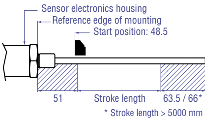
G-Series GH with block magnet
