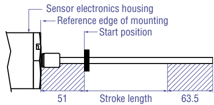
G-Series GT2 / GT3 with U- / ring-magnet
