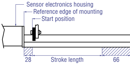
G-Series GP with block magnet
