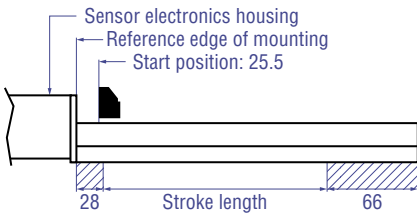
G-Series GH with block magnet
